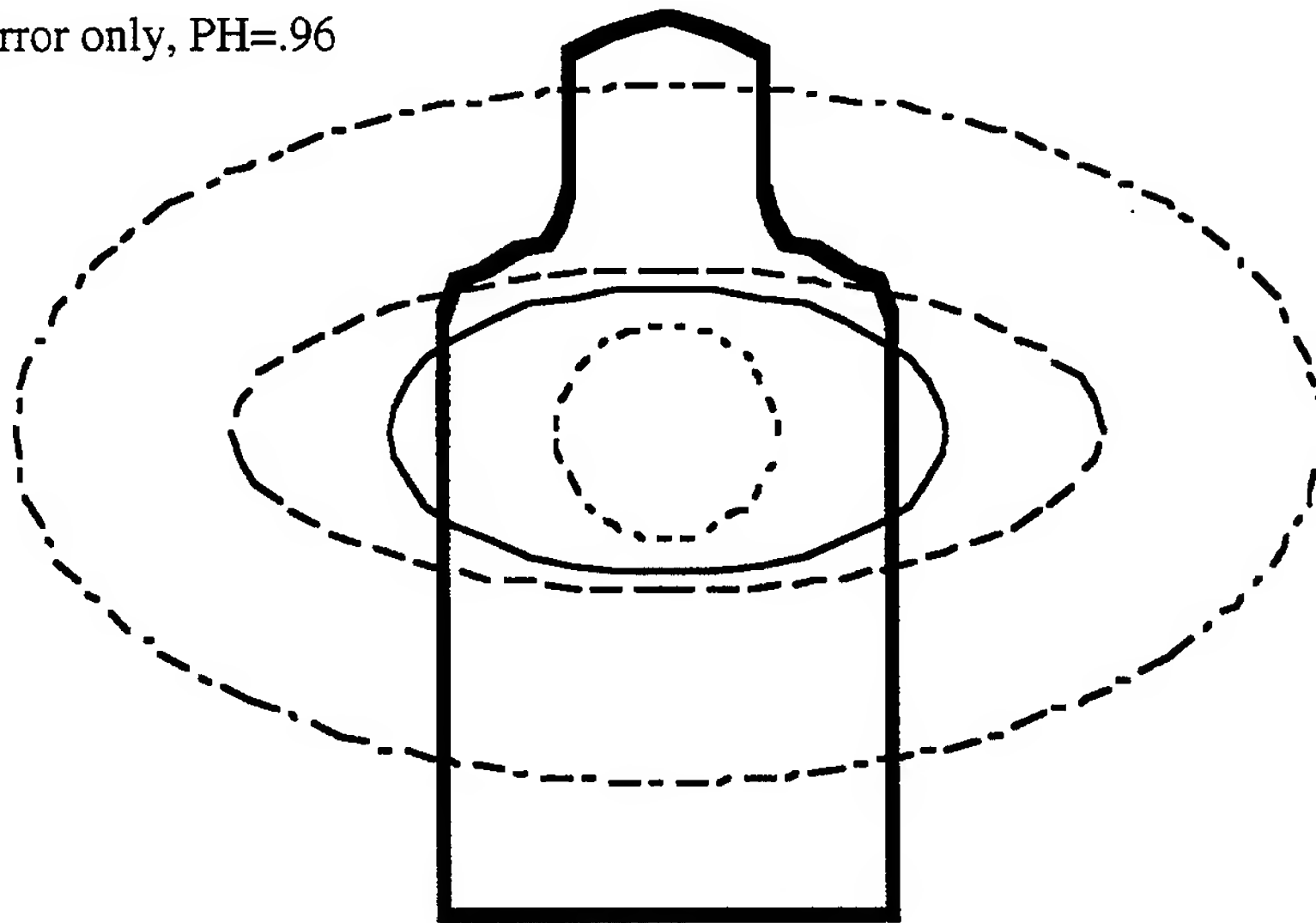
Figure 10. Total Errors. .300 WM, 700 m.
